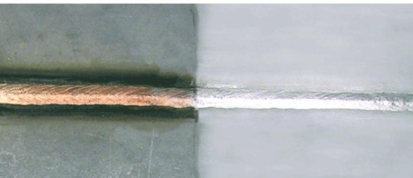
Before and after pickling. Avesta Pickling Paste 101 – for brush pickling in all positions.
